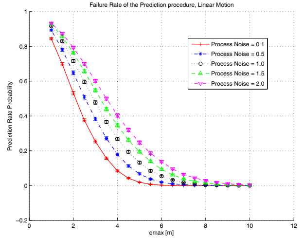
Fig. 2. Failure rate of the prediction procedure, with linear motion, for different levels of process noise.
